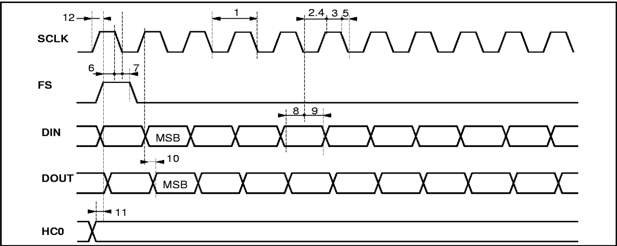
Figure 9 : Serial Interface Timing Diagram
