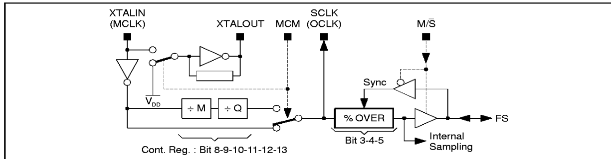
Figure 1 : Clock Block Diagram
