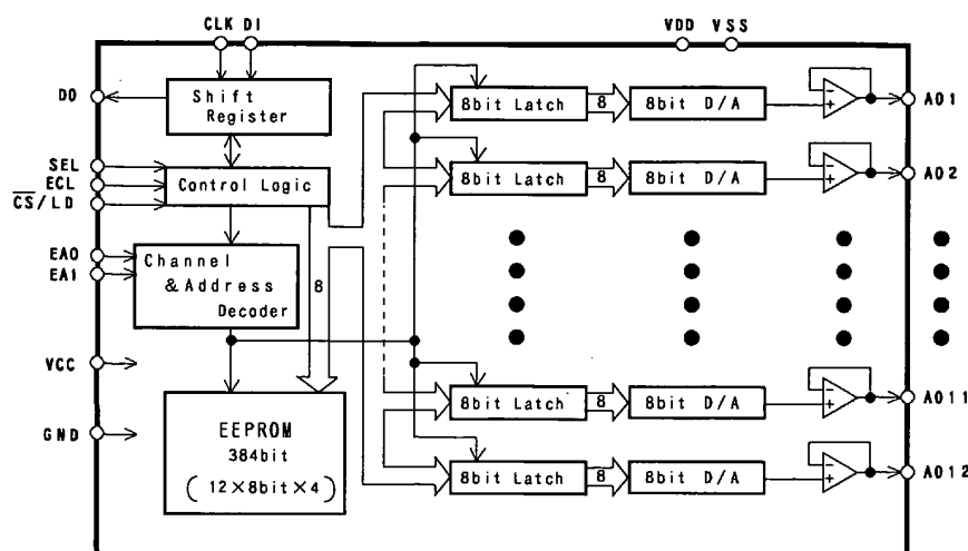
Block Diagram
