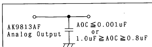
•Load Circuit-A
