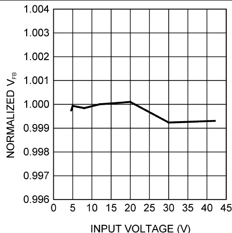
Figure 16. Normalized Feedback Voltage vs Input Voltage
