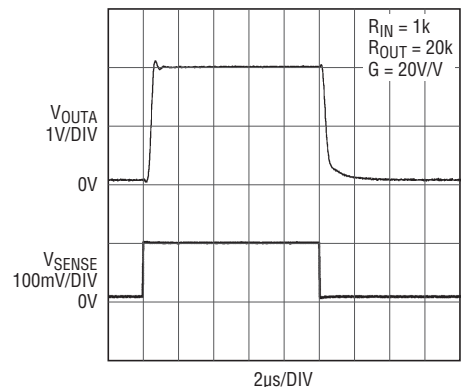
Amplifier Step Response ( V_{\text{SENSE}} = 10\text{mV} to 100mV)
