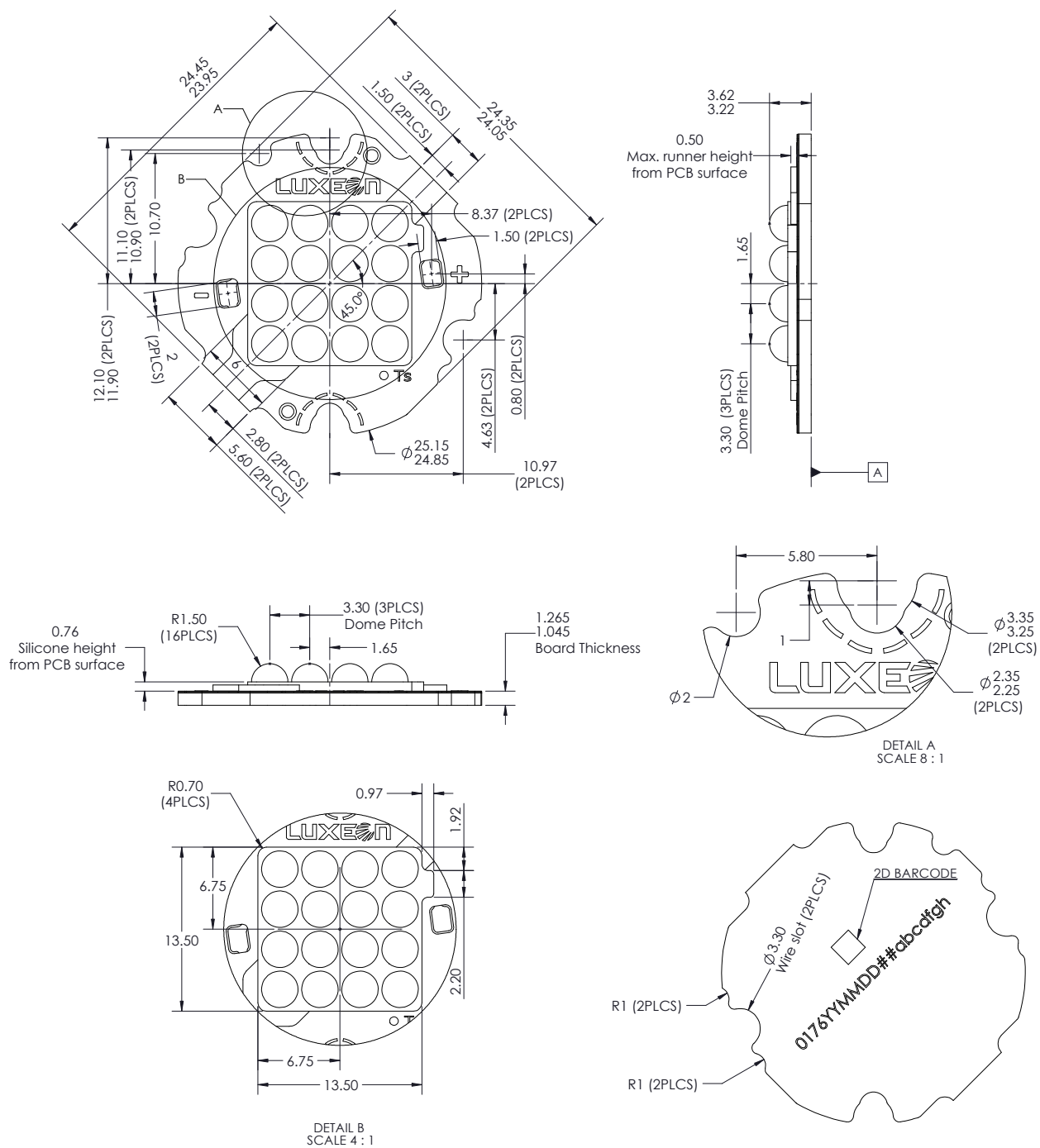
Figure 6. Dimensions for LXXx-Pxxx-xx16(A).
