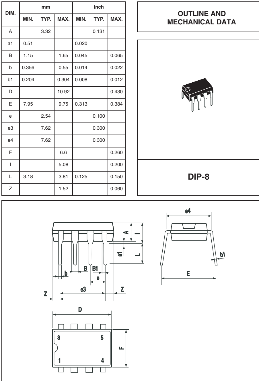
Figure 27. DIP-8 Mechanical Data & Package Dimensions
