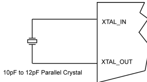
Figure 7. Crystal Input Interface
