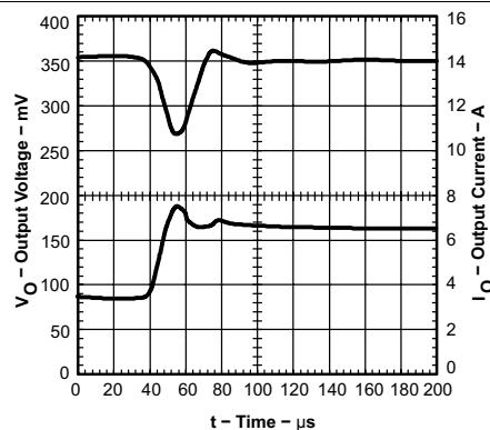
Figure 14. Transient Response
