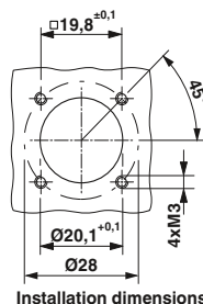
Installation dimensions
