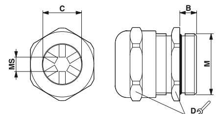
Dimensional drawing: HC-EMV-KV-M...
