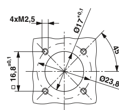
Installation dimensions
