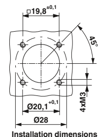
Installation dimensions
