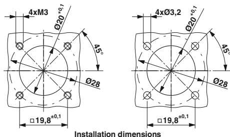
Installation dimensions
