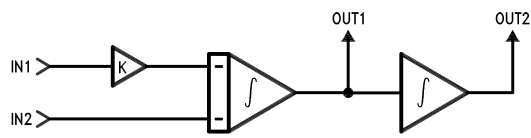
Equivalent Circuit
