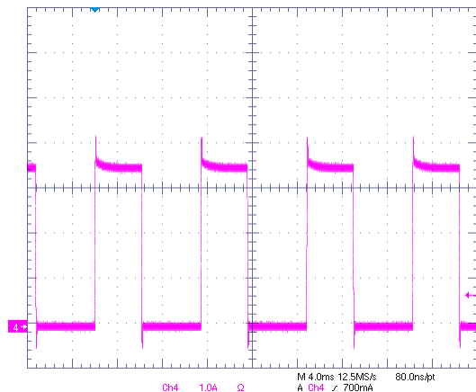
VIN=2.5V, VCNTL=3.3V, VOUT=1.25V, VOUT short to GND
