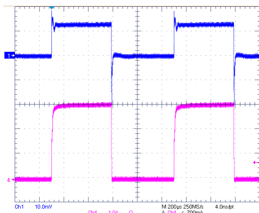
VIN=1.2V, VCNTL=5V, VOUT=0.6V @ 3A Sinking
