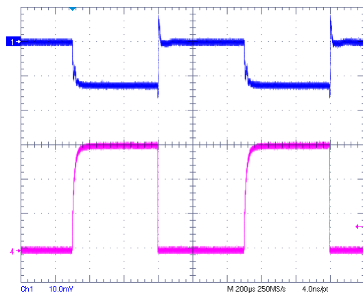
VIN=1.5V, VCNTL=5V, VOUT=0.75V @ 3A Sourcing
