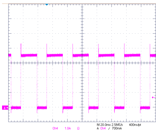
VIN=1.8V, VCNTL=3.3V, VOUT=0.9V, VOUT short to VIN
