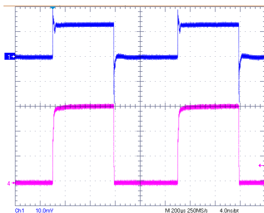
VIN=1.5V, VCNTL=5V, VOUT=0.75V @ 3A Sinking
