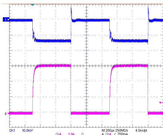
VIN=1.2V, VCNTL=3.3V, VOUT=0.6V @ 3A Sourcing
