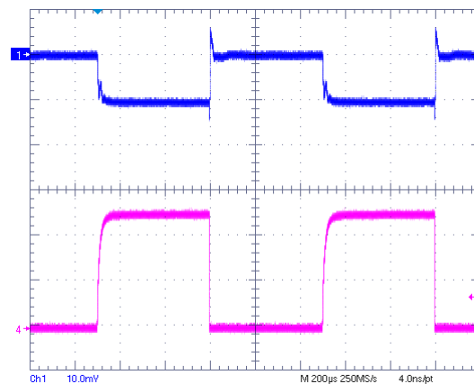
VIN=1.5V, VCNTL=5V, VOUT=0.75V @ 2.5A Sourcing
