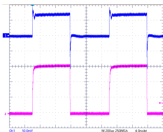
VIN=1.2V, VCNTL=3.3V, VOUT=0.6V @ 3A Sinking
