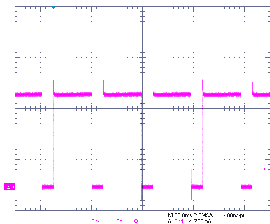
VIN=1.5V, VCNTL=3.3V, VOUT=0.75V, VOUT short to GND
