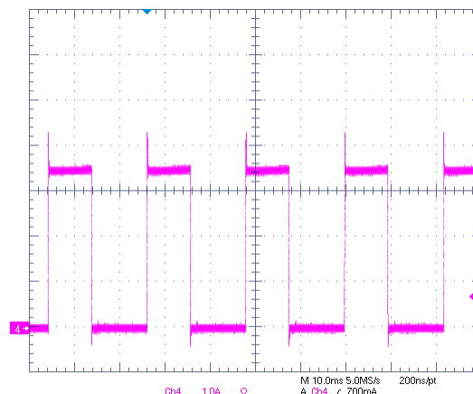
VIN=2.5V, VCNTL=5V, VOUT=1.25V, VOUT short to VIN
