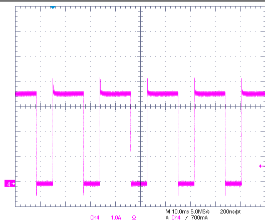
VIN=1.8V, VCNTL=3.3V, VOUT=0.9V, VOUT short to GND
