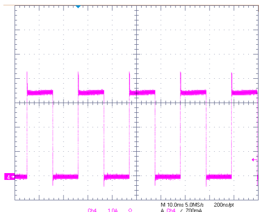
VIN=2.5V, VCNTL=3.3V, VOUT=1.25V, VOUT short to VIN
