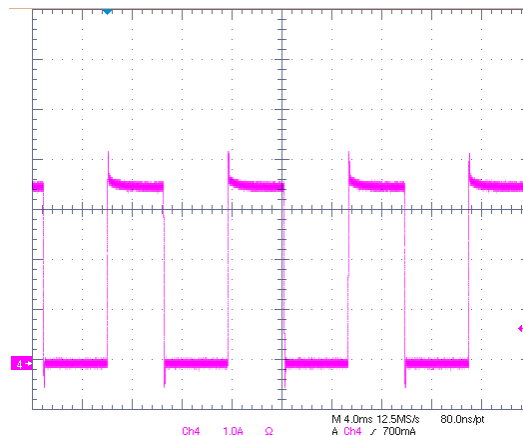
VIN=2.5V, VCNTL=5V, VOUT=1.25V, VOUT short to GND
