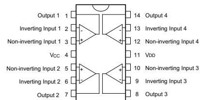
TS974ID-TS974IDT (SO-14) TS974IPT (TSSOP14)
