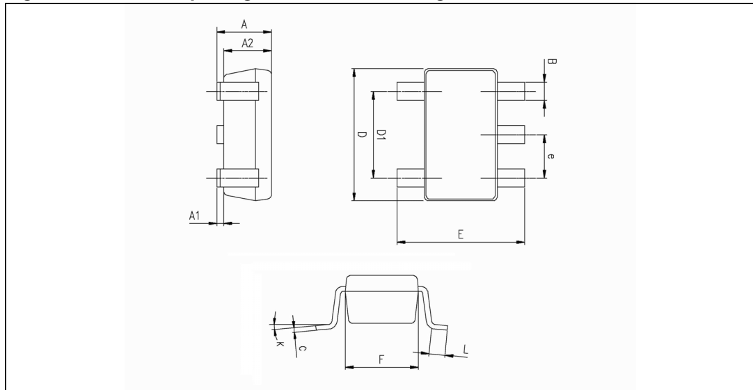
Figure 13. SOT23-5 package mechanical drawing
