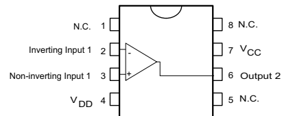
TS972ID-TS972IDT (SO-8) TS972IPT (TSSOP8)
