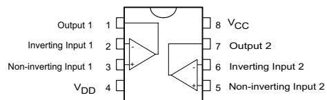
TS972IQT (DFN8)
