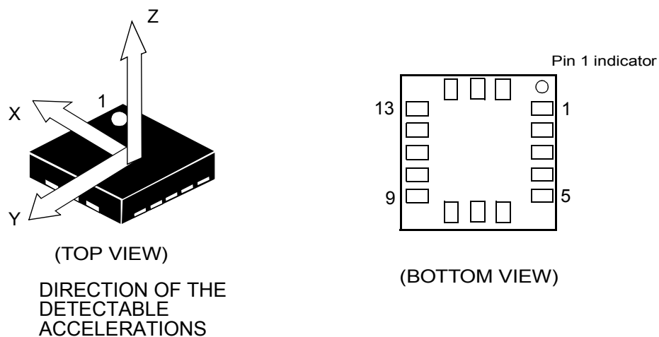
Figure 2. Pin connections
