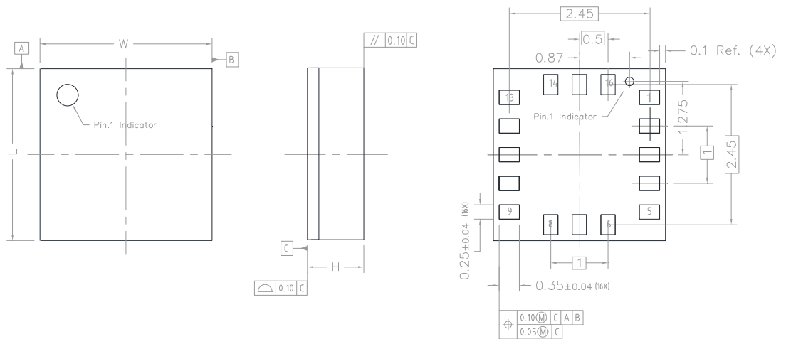
Figure 12. TFLGA-16L 3 x 3 x 1.0 mm package outline and mechanical data
