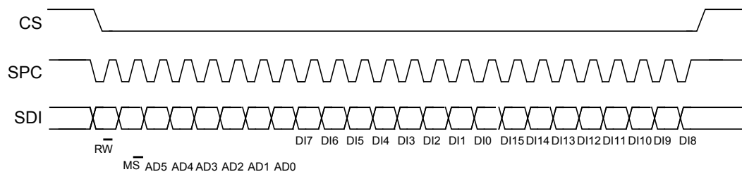
Figure 10. Multiple byte SPI write protocol (2-byte example)
