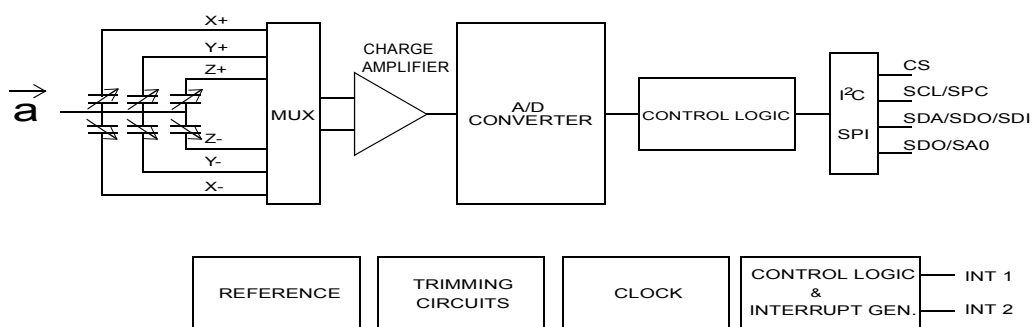
Figure 1. Block diagram
