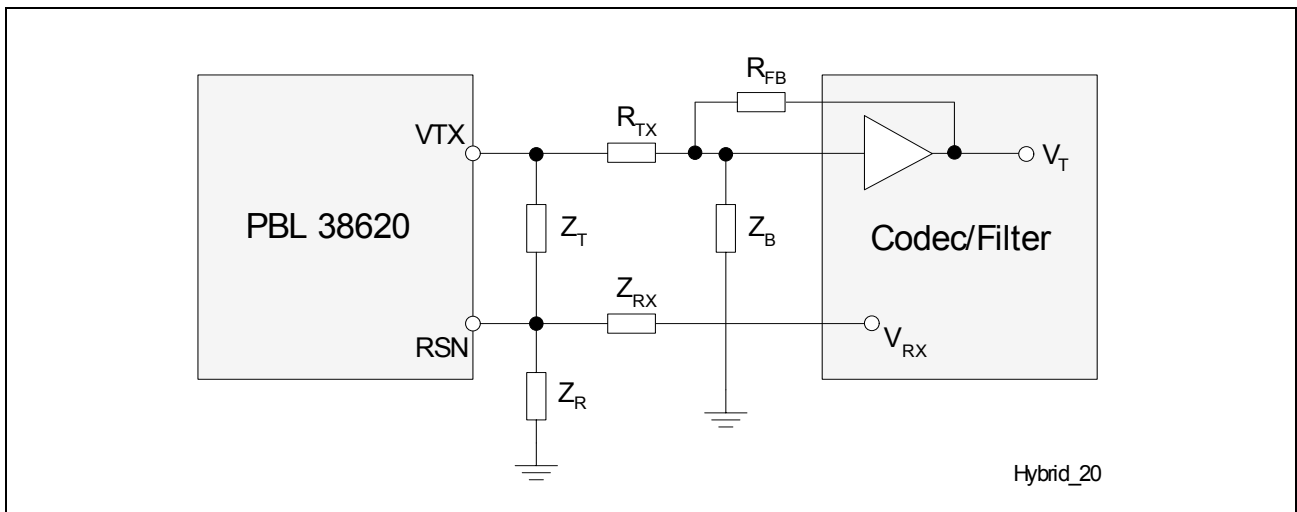
Figure 10 Hybrid Function
