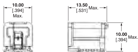
Surface Mount Jack Receptacle
