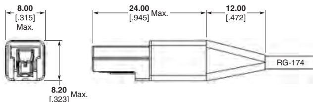
Cable Plug
