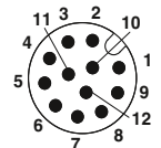
Plug, 12-pos.
