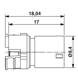
M12 contact carrier
