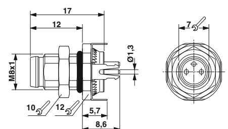
M8 flush-type plug, straight,
