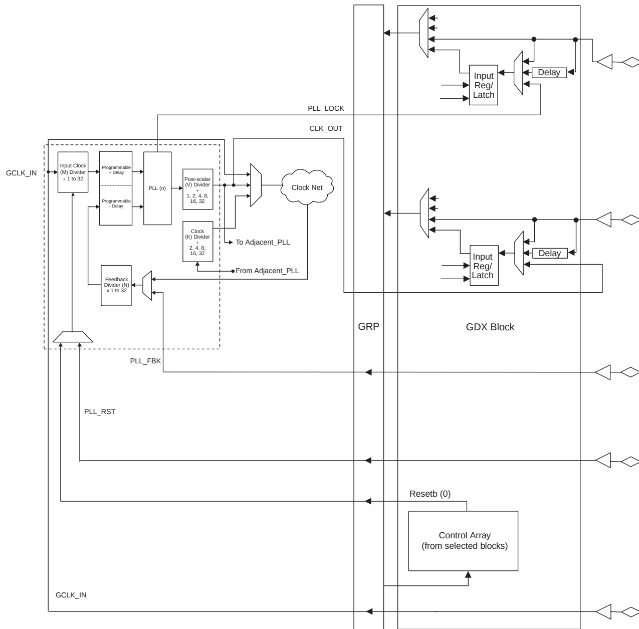
Figure 7. I/O Pin Connection to the sysCLOCK PLL 1
