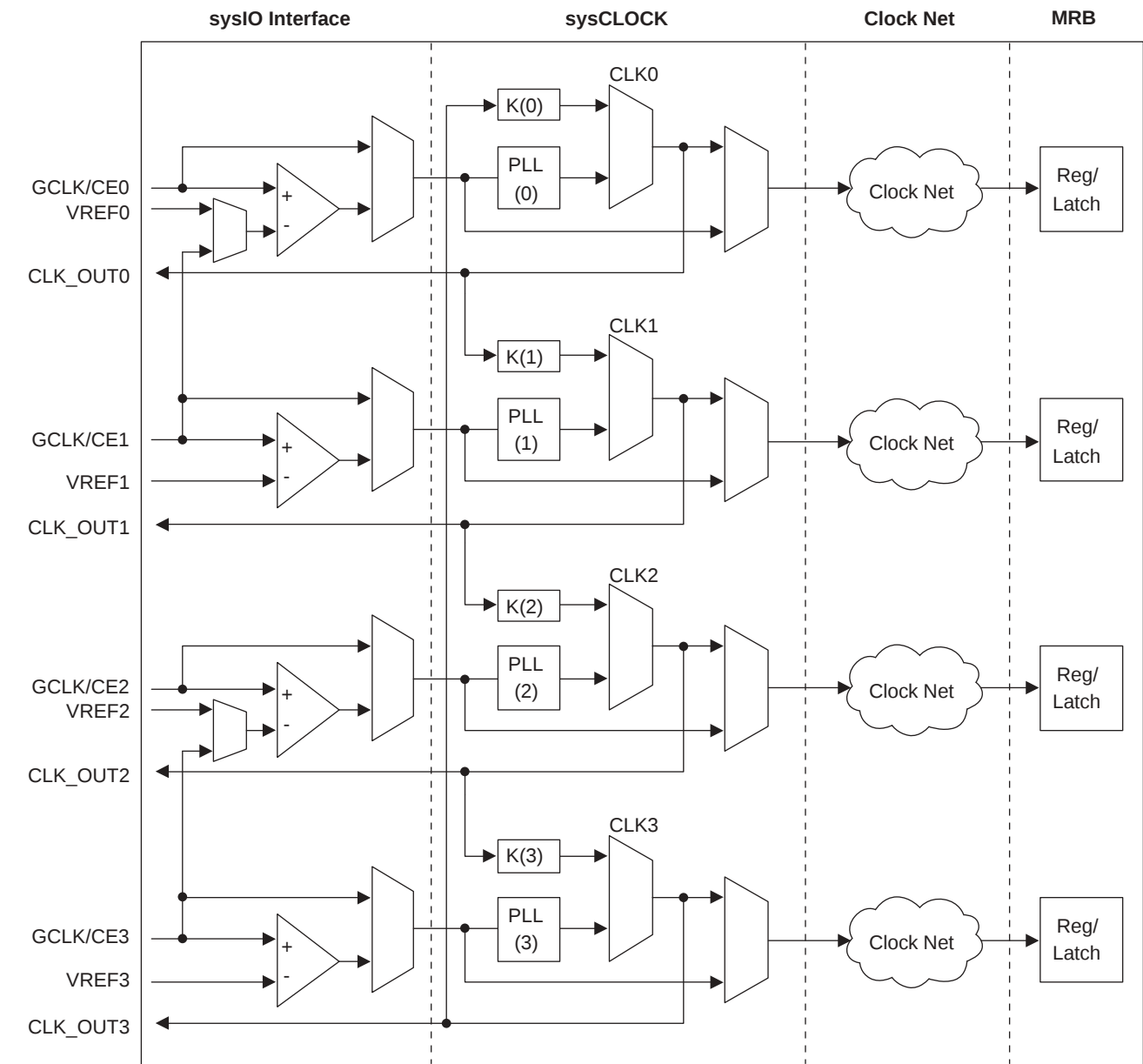
Figure 8. ispGDX2-256 CLOCK Network
