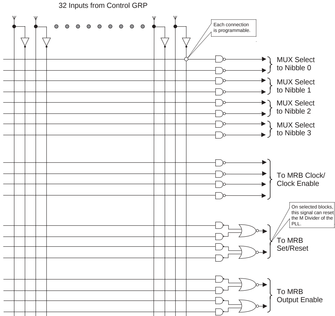
Figure 4. ispGDX2 Family Control Array
