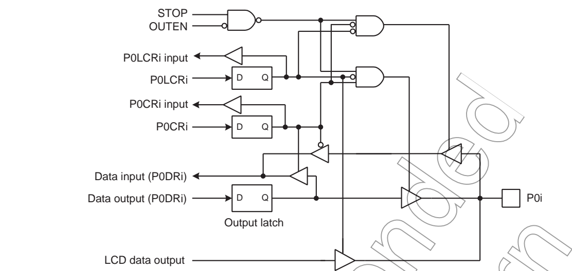
Figure 5-2 Port 0
