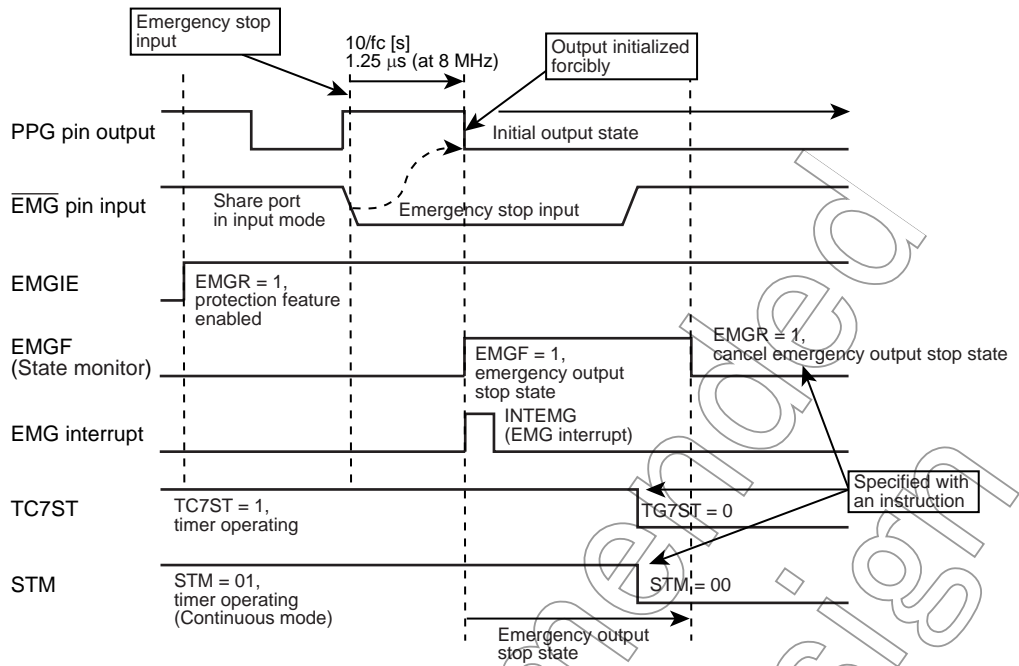
Figure 8-23 Timing between \overline{\text{EMG}} Pin Input being Detected and PPG Outputs being Disabled
