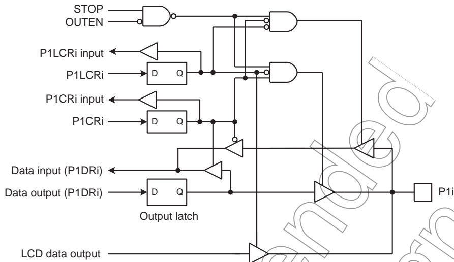
Figure 5-3 Port 1
