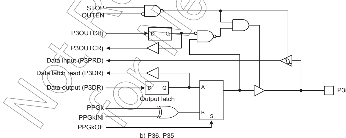
Figure 5-5 Port 3
