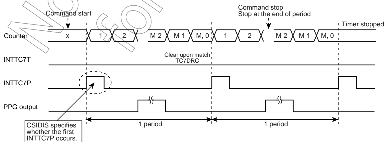
Figure 8-21 Period Interrupt
