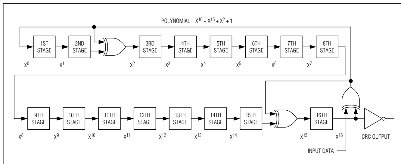
Figure 13. CRC-16 Hardware Description and Polynomial
