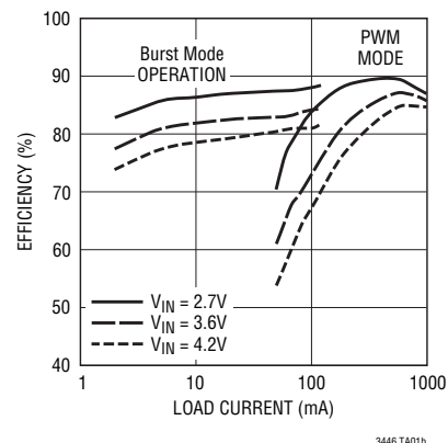
Buck Efficiency vs Buck Load Current
