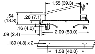
Mounting Holes
