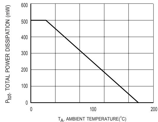
Figure1 Total Power Dissipation vs. Ambient Temperature
