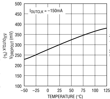
V_{OUTCLK} Dropout Voltage vs Temperature
