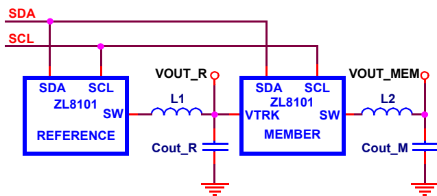
FIGURE 17. PMBus TRACKING
