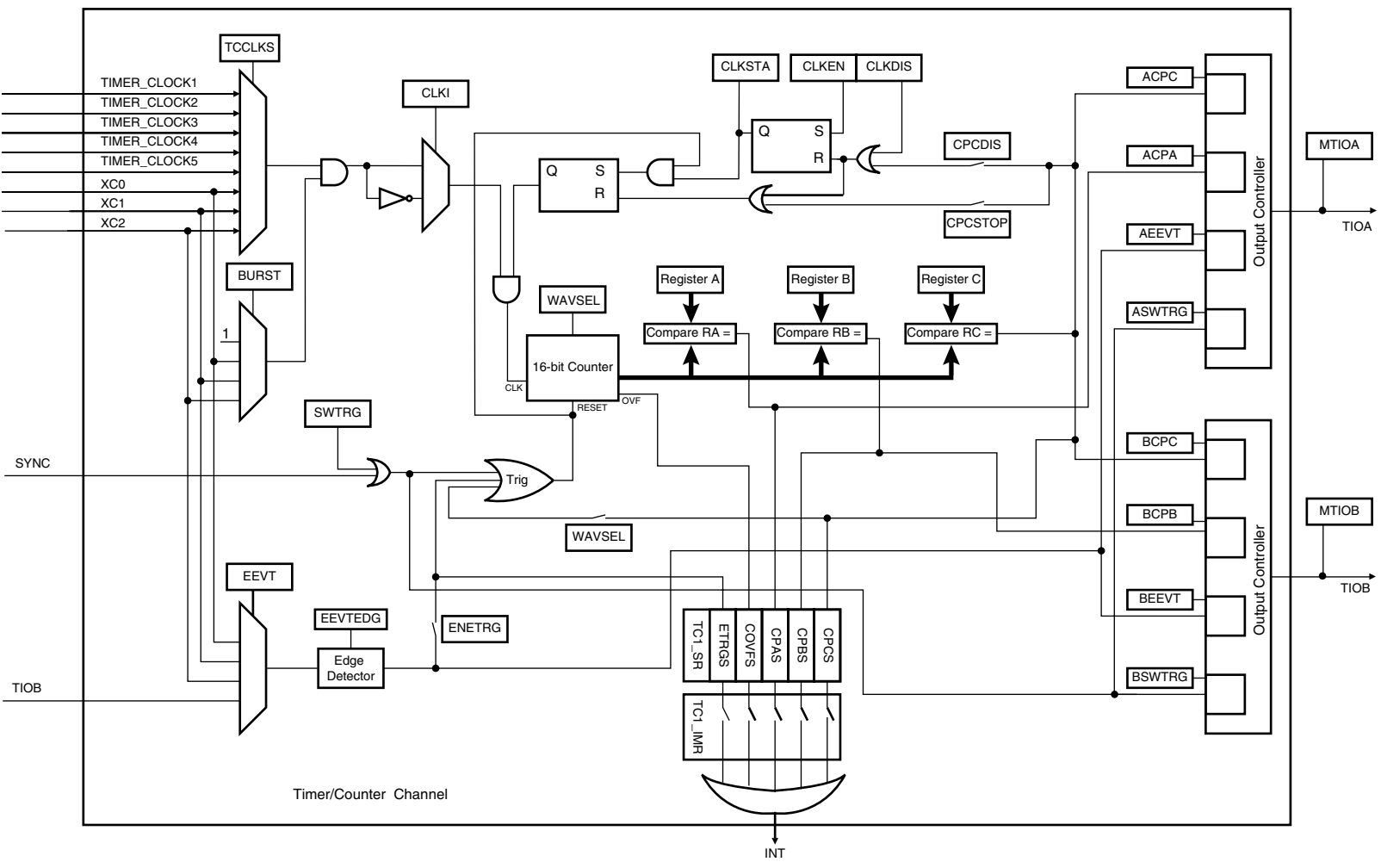
Figure 33-5. Waveform Mode
