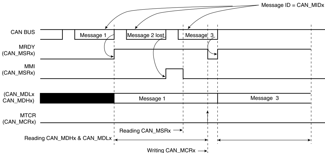
Figure 39-11. Receive Mailbox
