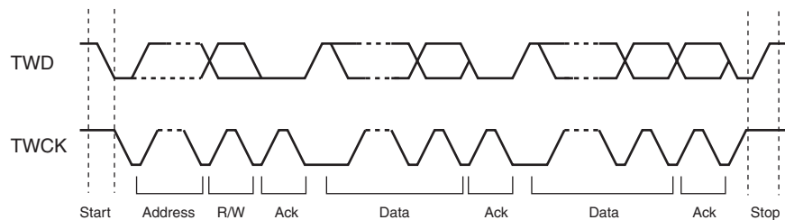
Figure 30-4. Transfer Format
