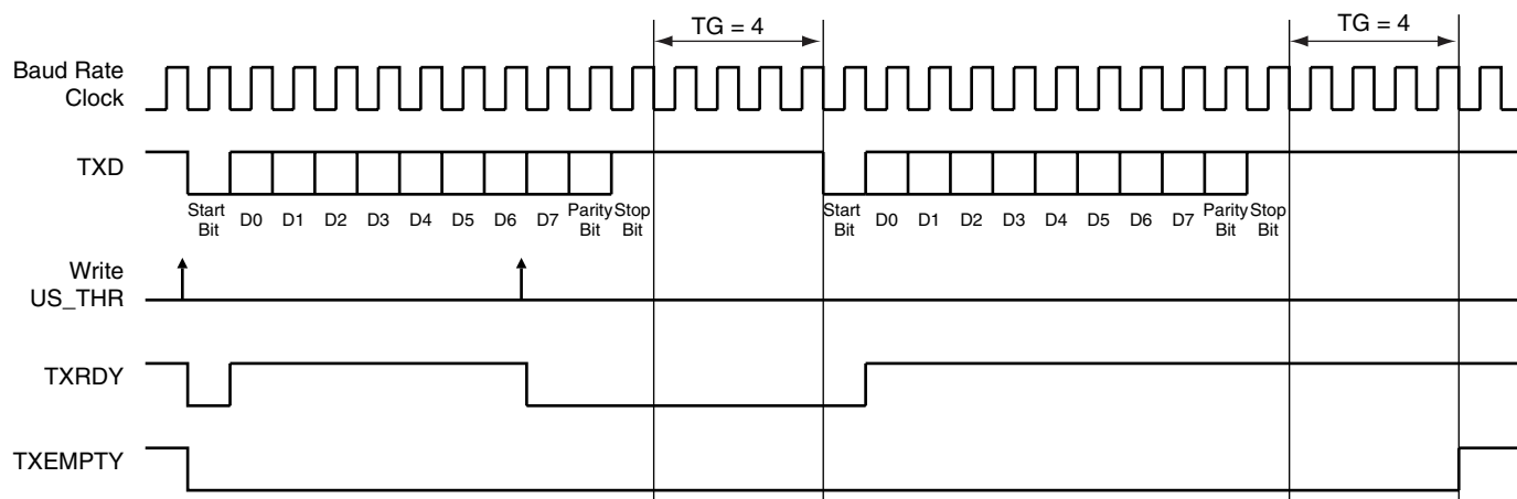
Figure 31-23. Timeguard Operations
