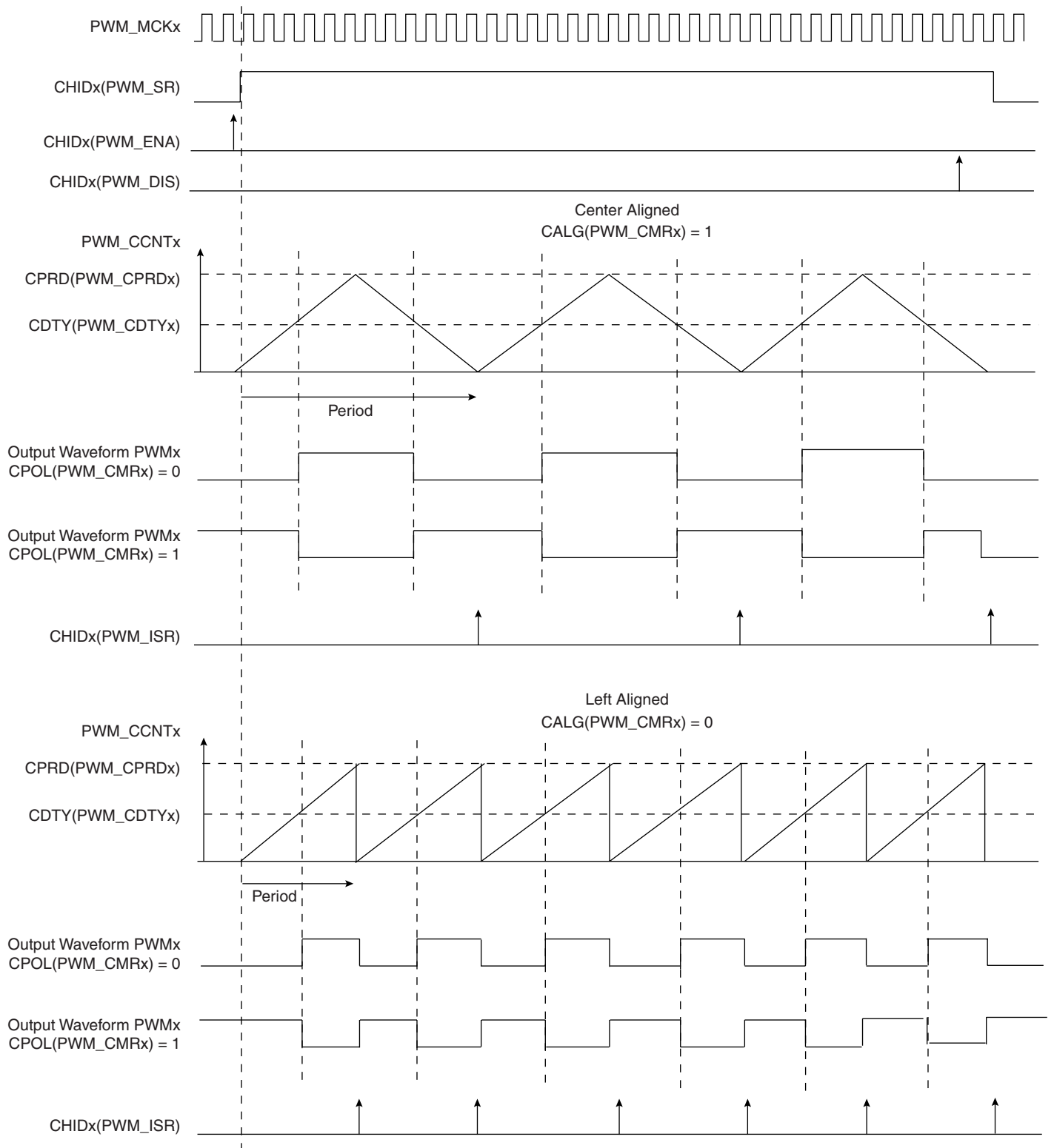
Figure 34-5. Waveform Properties
