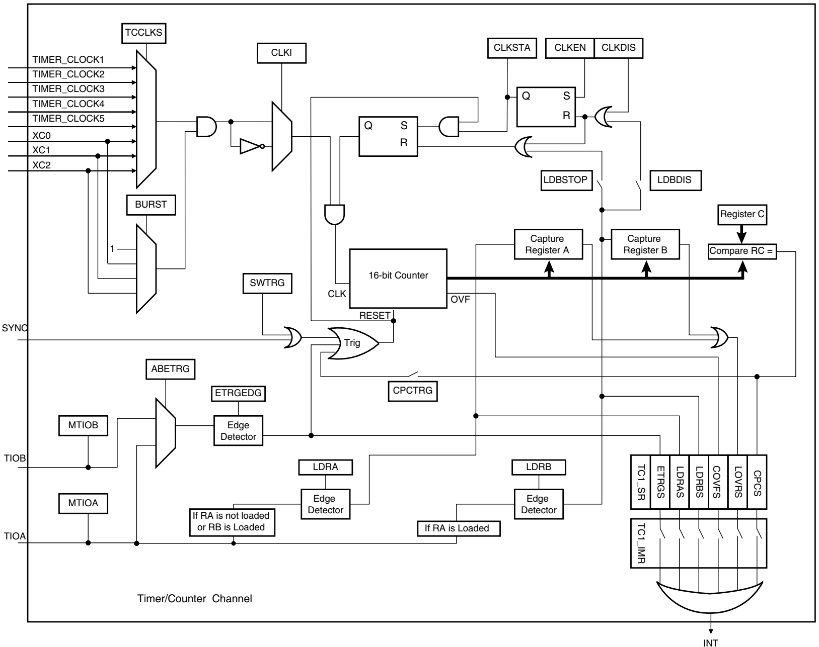
Figure 33-4. Capture Mode
