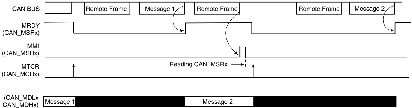
Figure 39-17. Producer Handling
