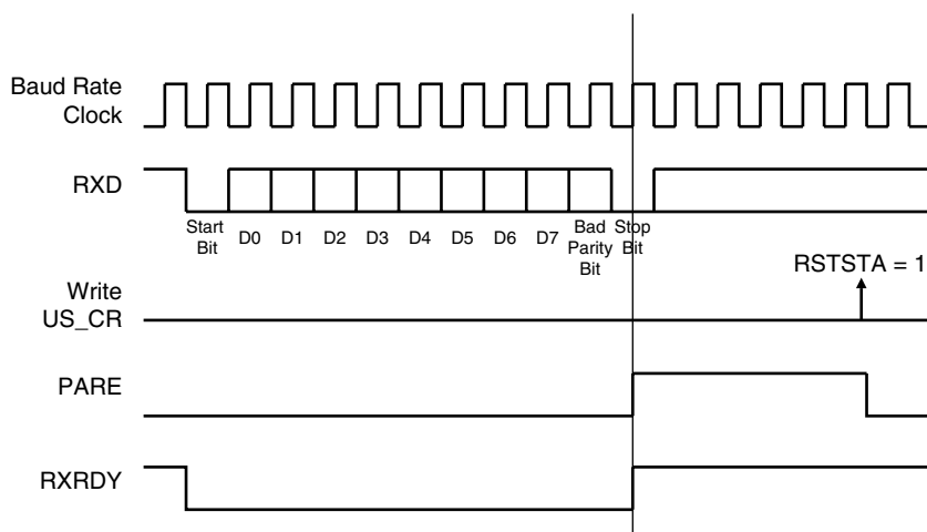
Figure 31-22. Parity Error
