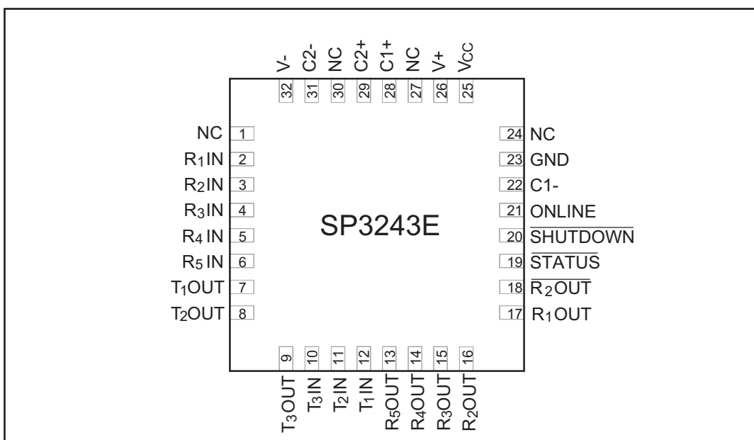
Figure 9. SP3243E QFN Pinout Configuration
