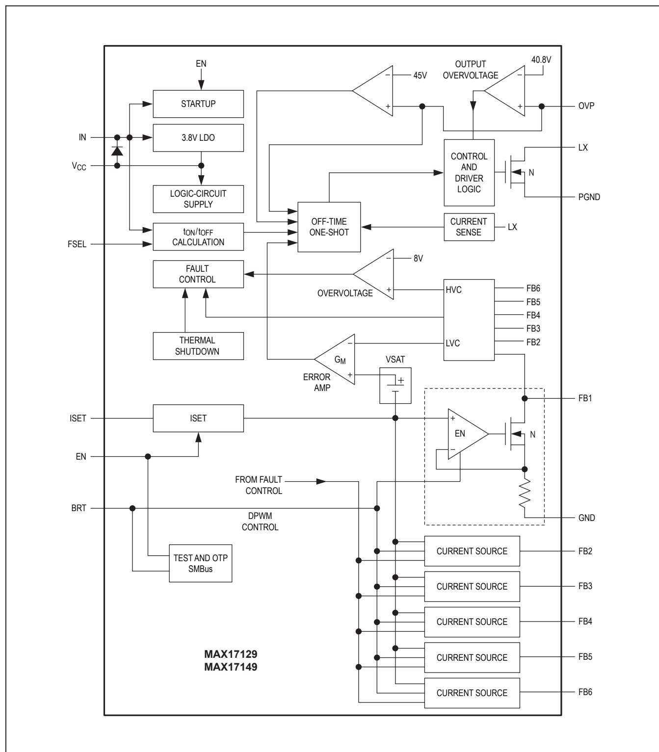
Figure 2. Functional Diagram
