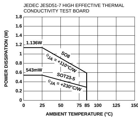
FIGURE 49. PACKAGE POWER DISSIPATION vs AMBIENT TEMPERATURE
