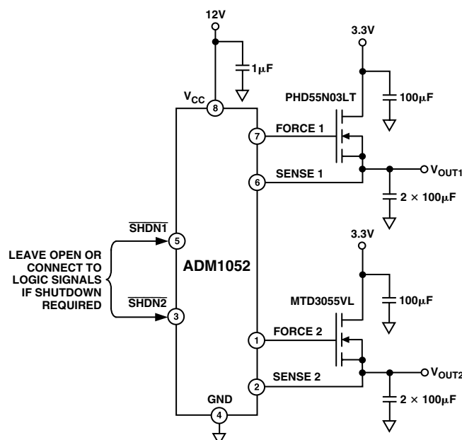
Figure 1. Test Circuit
