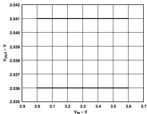
TPC 3. Line Regulation, Channel 2
