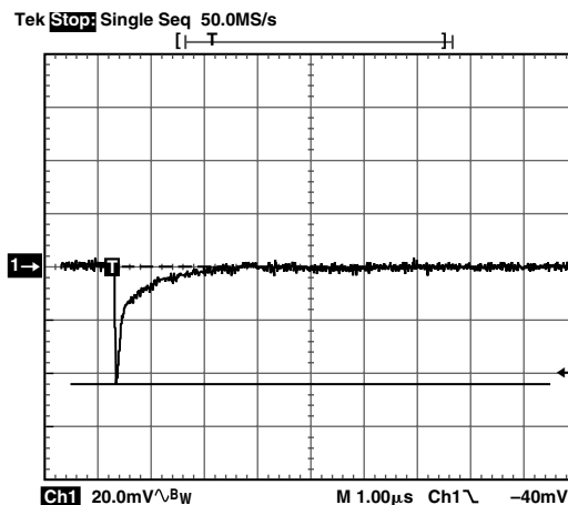
TPC 10. Transient Response Channel 2, 10 mA to 2 A Output Load Step
