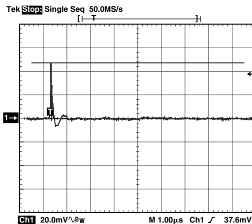
TPC 11. Transient Response Channel 2, 2 A to 10 mA Output Load Step
