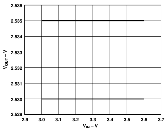
TPC 2. Line Regulation, Channel 1
