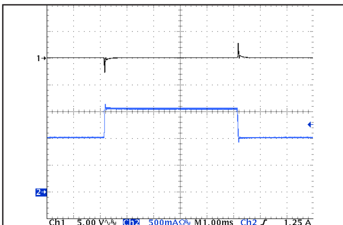
Figure 5: Output voltage response to step-change in load current (66%-100%-66% of I out (max); dI/dt = 0.05 A/μs). Load cap: 1 μF ceramic capacitor. Ch 1: V out (5 V/div), Ch 2: I out (500 mA/div).
