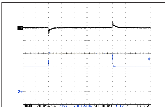
Figure 5: Output voltage response to step-change in load current (66%-100%-66% of Iout(max); dI/dt = 0.1 A/μs). Load cap: 1 μF ceramic and 15 μF tantalum capacitors. Ch 1: Vout (200 mV/div), Ch 2: Iout (5 A/div).
