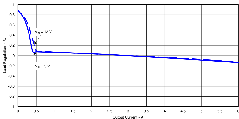
Figure 4-3. TPS54628EVM-052 Load Regulation, V_{IN} = 5\text{ V} and V_{IN} = 12\text{ V} .
