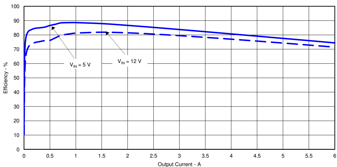
Figure 4-1. TPS54628EVM-052 Efficiency
