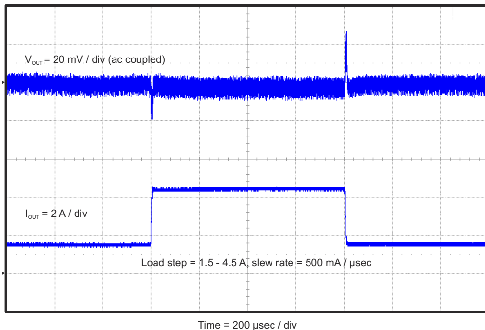
Figure 4-5. TPS54628EVM-052 Load Transient Response
