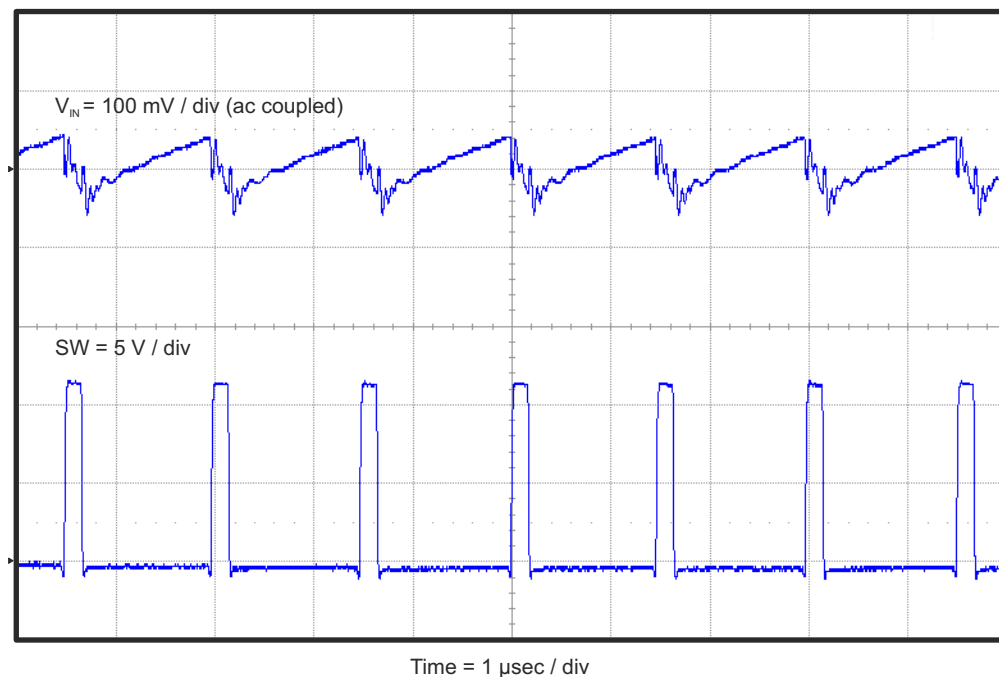
Figure 4-9. TPS54628EVM-052 Input Voltage Ripple
