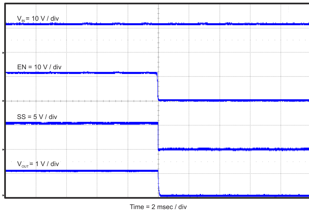
Figure 4-13. TPS54628EVM-052 Shut-Down Relative to EN with SS
