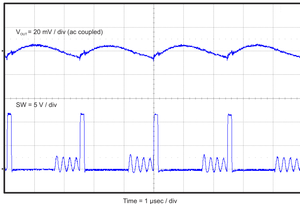
Figure 4-7. TPS54628EVM-052 Output Voltage Ripple ( I_{OUT} = 300 \text{ mA} )
