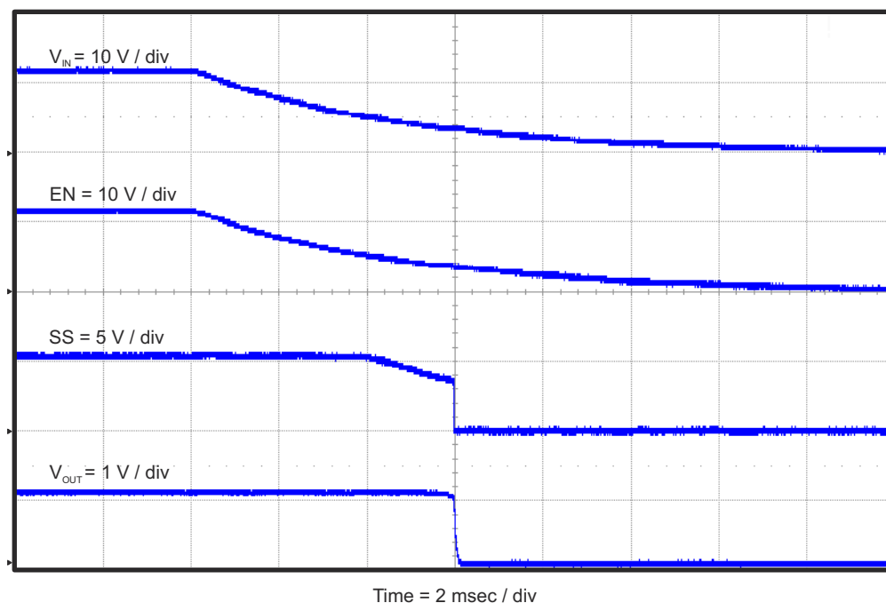
Figure 4-12. TPS54628EVM-052 Shut-Down Relative to V_{IN} with SS
