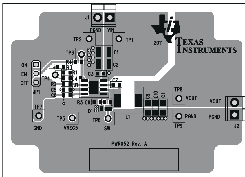
Figure 5-1. Top Assembly
