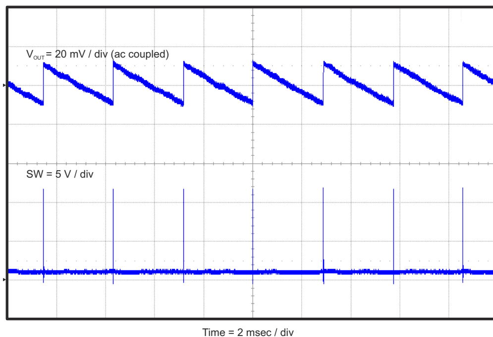
Figure 4-8. TPS54628EVM-052 Output Voltage Ripple ( I_{OUT} = 0.2 \text{ mA} )
