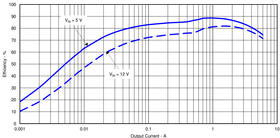
Figure 4-2. TPS54628EVM-052 Light-Load Efficiency
