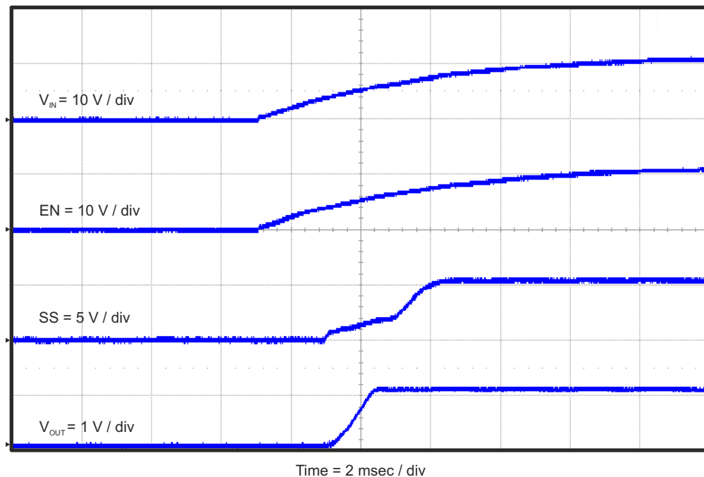
Figure 4-10. TPS54628EVM-052 Start-Up Relative to V_{IN} with SS
