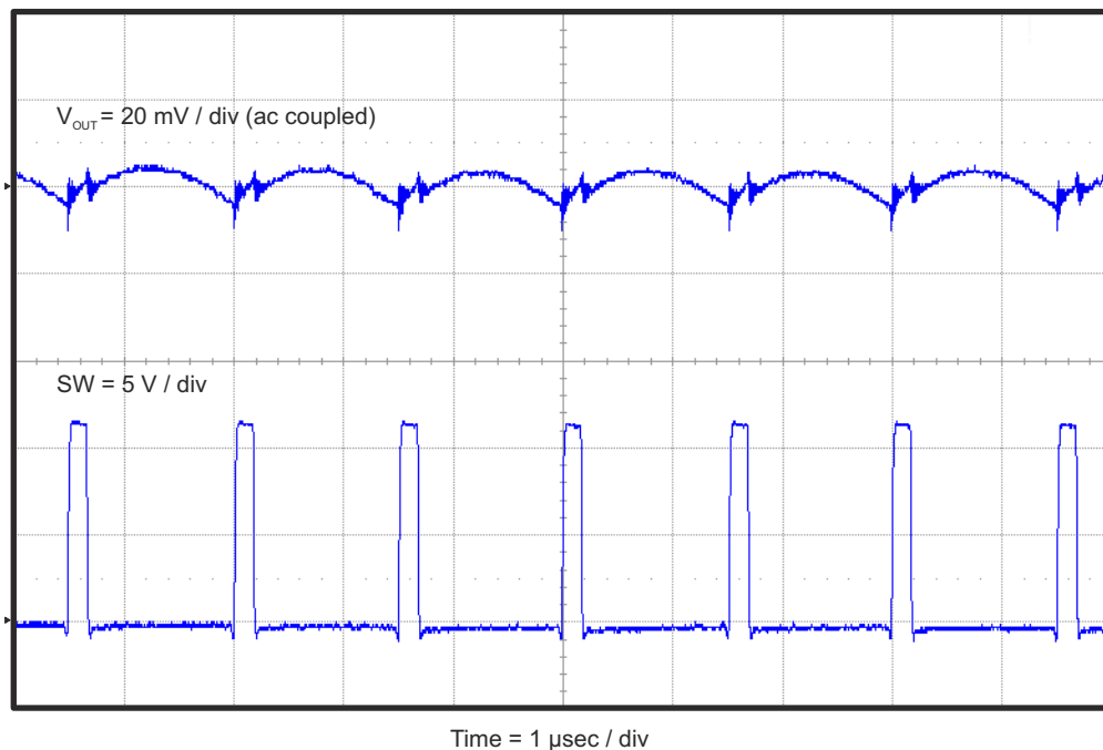
Figure 4-6. TPS54628EVM-052 Output Voltage Ripple ( I_{OUT} = 6 \text{ A} )
