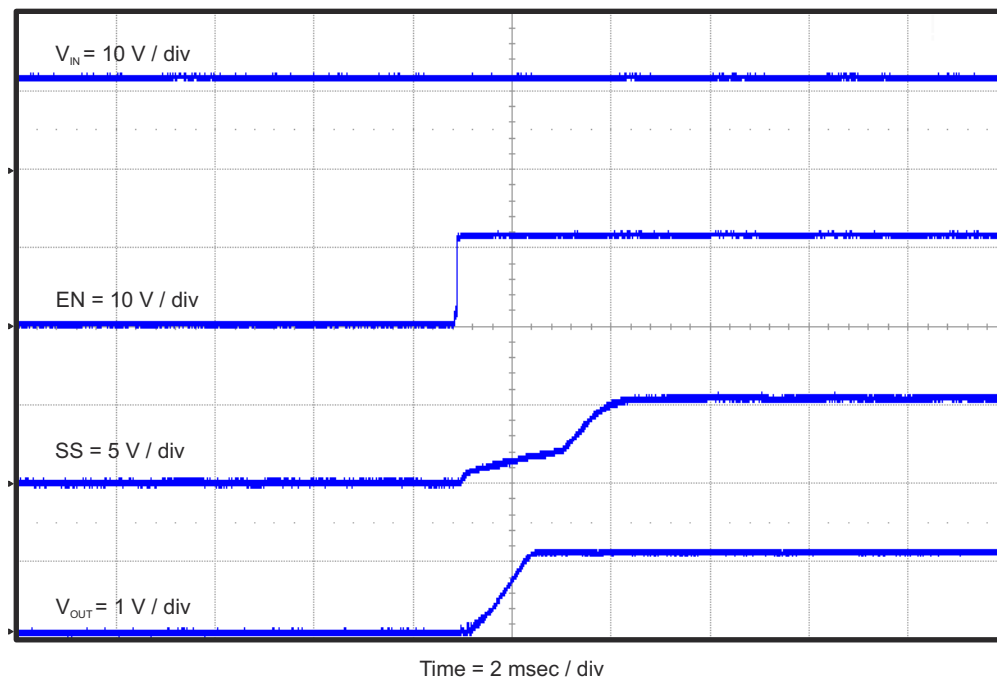
Figure 4-11. TPS54628EVM-052 Start-Up Relative to EN with SS
