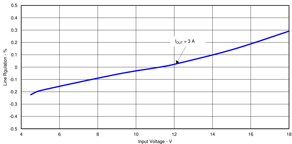
Figure 4-4. TPS54628EVM-052 Line Regulation
