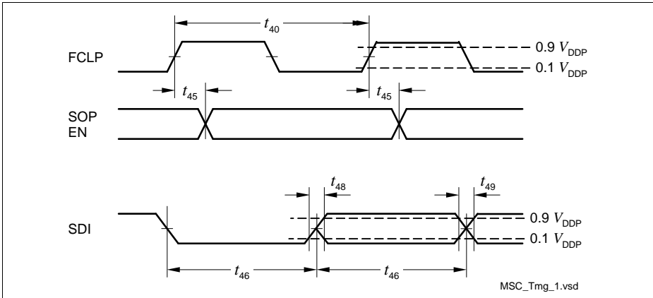
Figure 18 MSC Interface Timing
