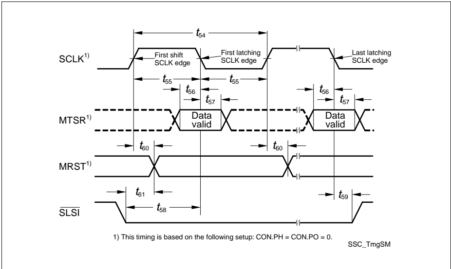
Figure 20 Slave Mode Timing
