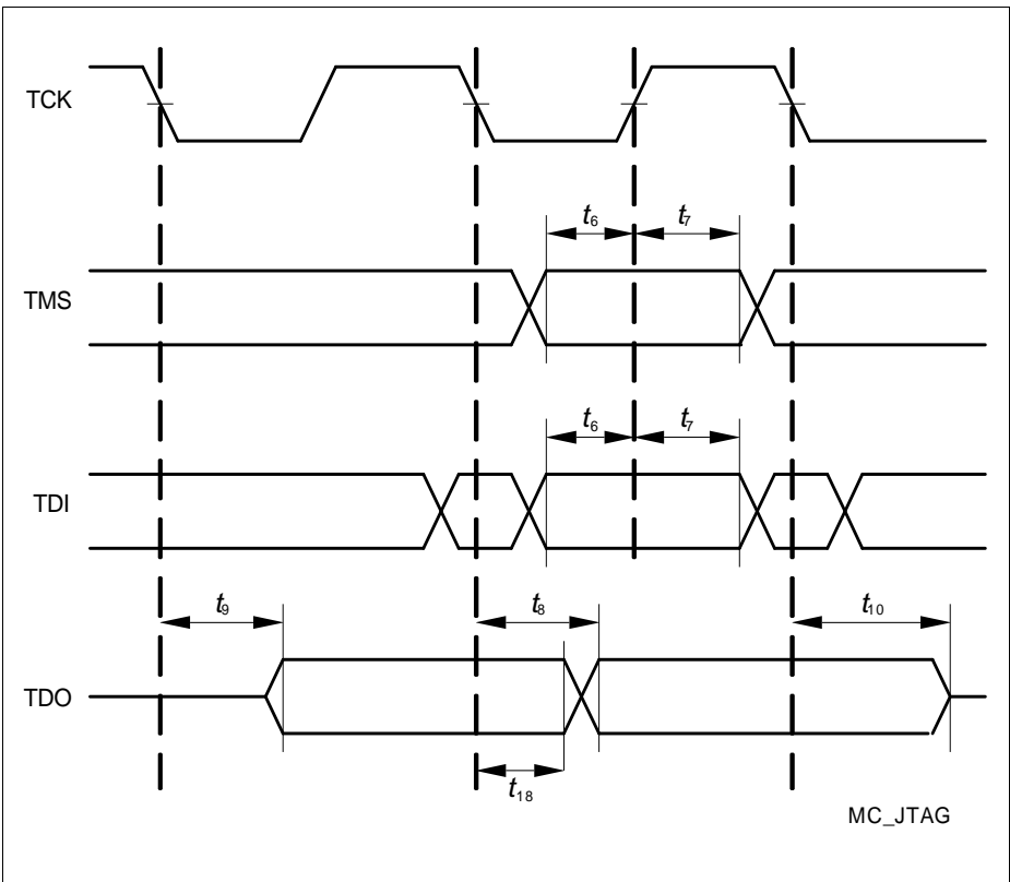
Figure 13 JTAG Timing
