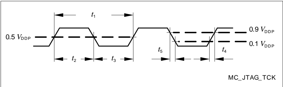
Figure 12 Test Clock Timing (TCK)
