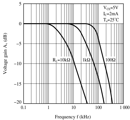
Fig.15 Frequency Response
