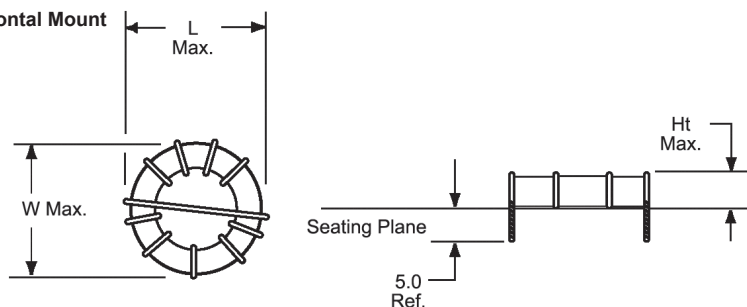
Figure 2 Horizontal Mount
