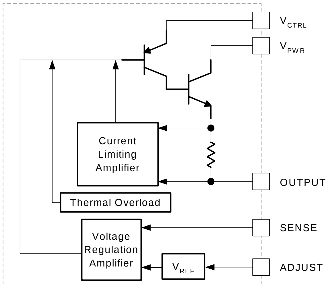
Figure 2 – Simplified Block Diagram
