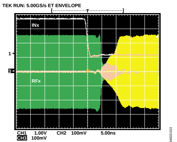
Figure 15. Switch Timing
