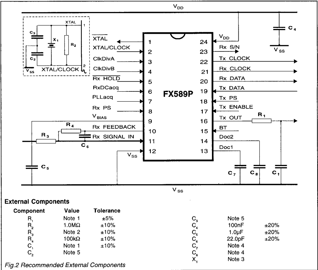
Fig.2 Recommended External Components
