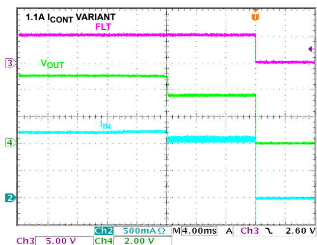
FIGURE 22. I_{LIM} WAVEFORM
