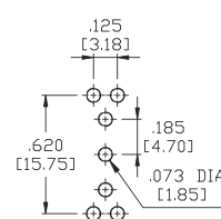
P.C.MOUNTING
