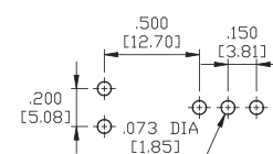
P.C.MOUNTING
