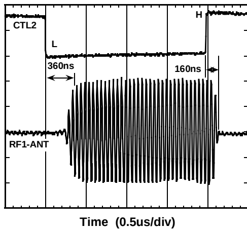
Switching Time
