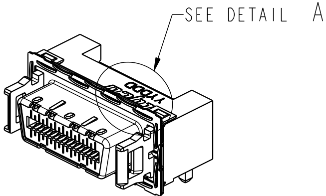
4X R/A RECEPTACLE ASSEMBLY WITHOUT MOUNTING TABS
