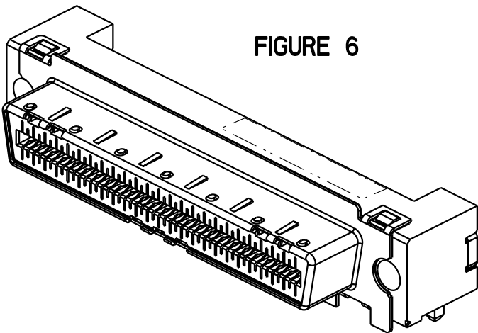
12X R/A RECEPTACLE ASSEMBLY
