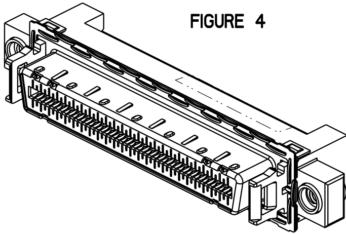
12X R/A RECEPTACLE ASSEMBLY WITH MOUNTING TABS
