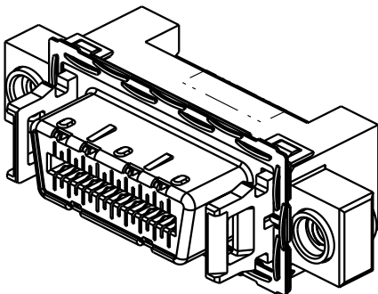
4X R/A RECEPTACLE ASSEMBLY WITH MOUNTING TABS
