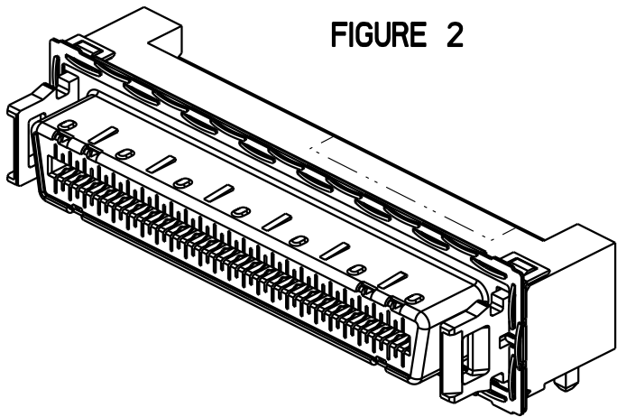
12X R/A RECEPTACLE ASSEMBLY WITHOUT MOUNTING TABS
