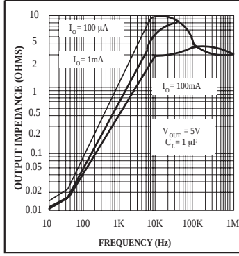
Output Impedance
