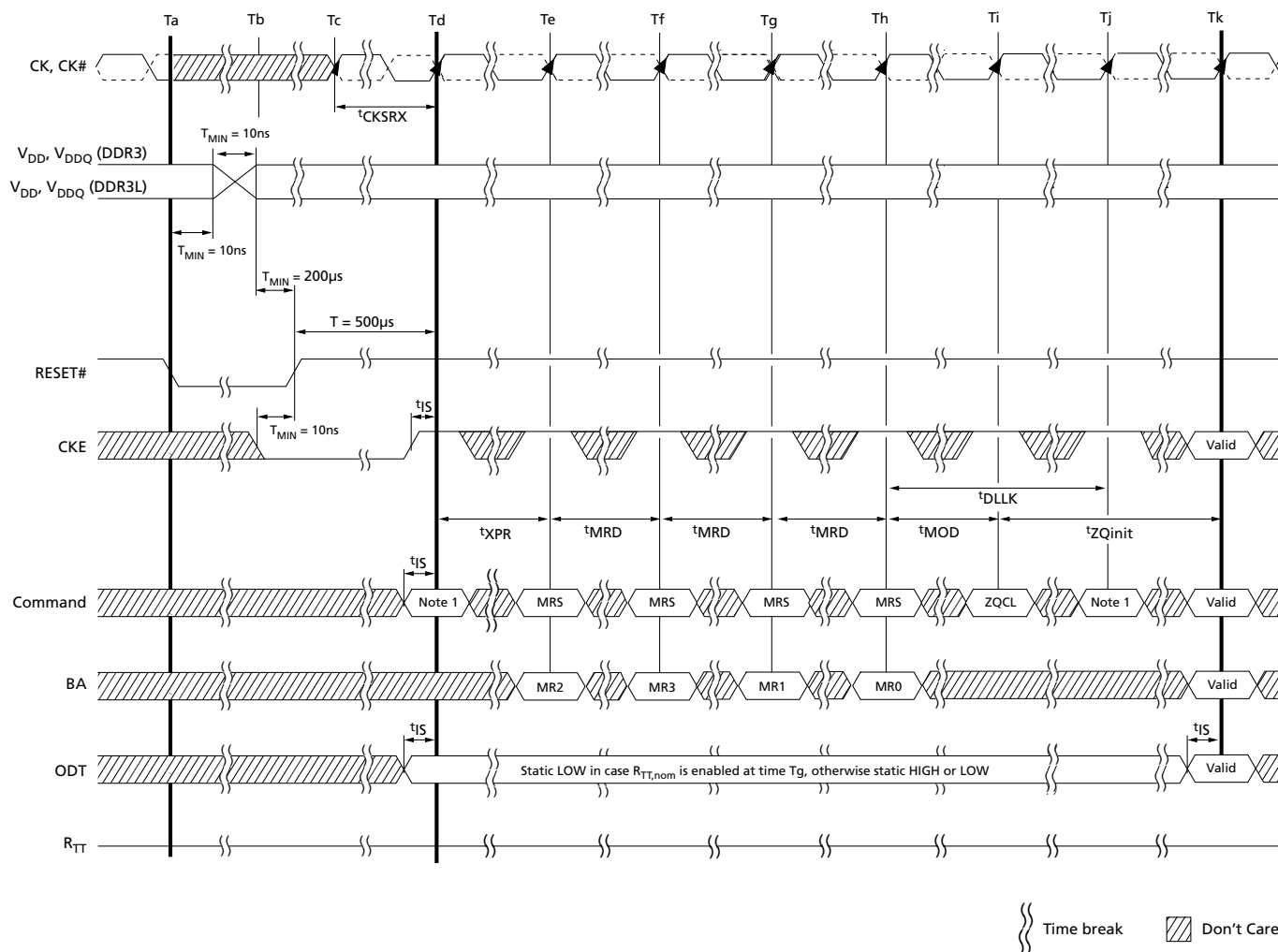
Figure 5: V DD Voltage Switching
