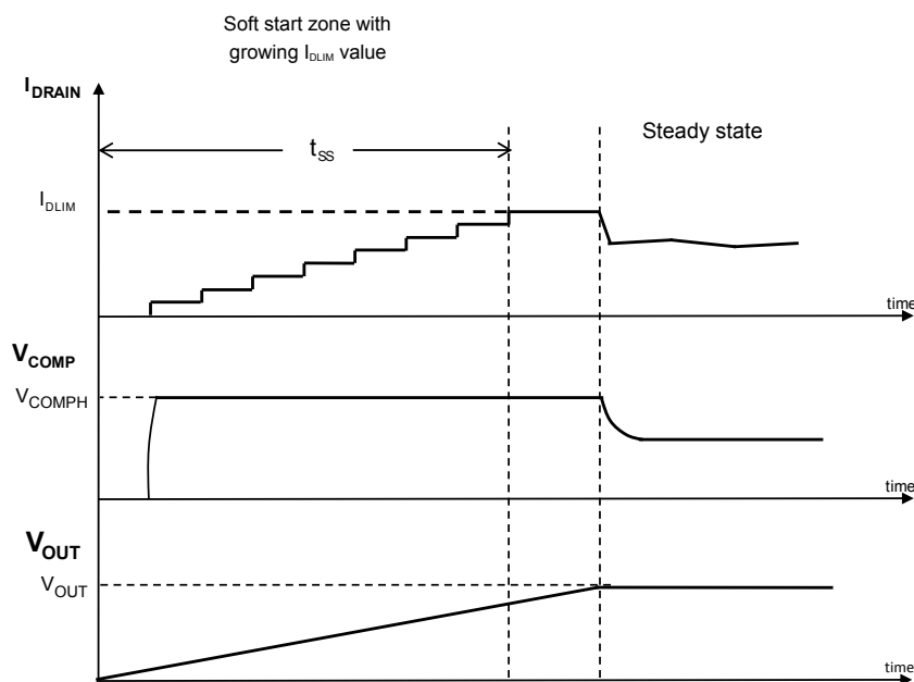
Figure 28. Soft startup
