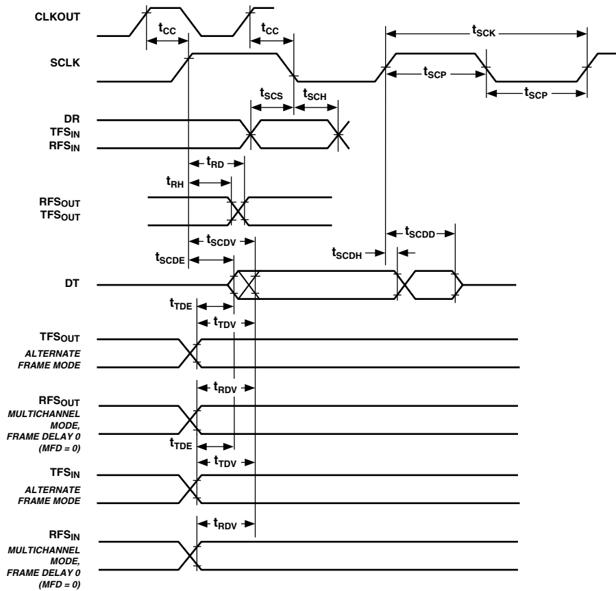
Figure 27. Serial Ports
