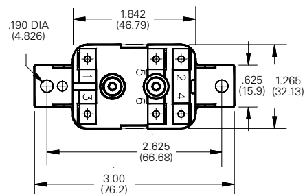
Standard I Bracket (Code 1)
