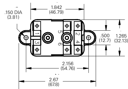
Special I Bracket (Code 0)
