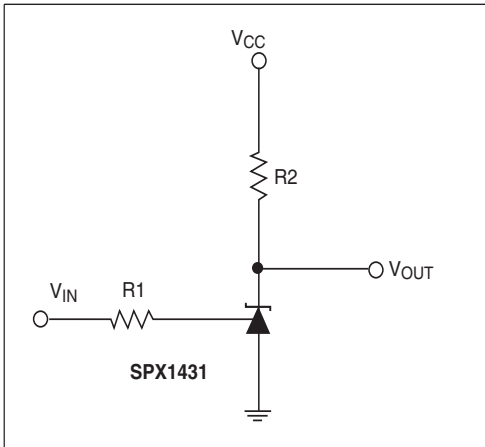
Figure 25. Single Supply Comparator with Temperature Compensated Threshold. V_{IN\text{ threshold}} = 2.5V
