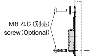
受け本体詳細 Catch body specifications
