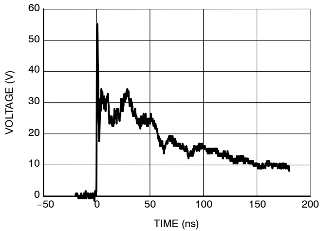
Figure 1. ESD5381MUT5G Clamping Voltage Screenshot Positive 8 kV Contact per IEC61000-4-2
