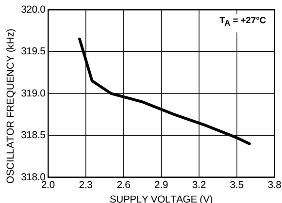
FIGURE 4. OSCILLATOR FREQUENCY vs SUPPLY VOLTAGE
