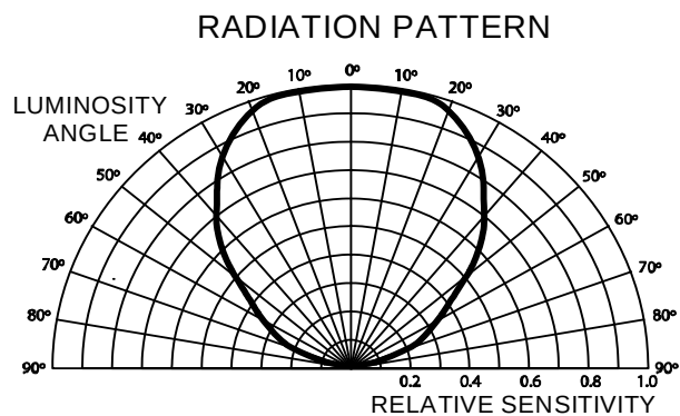
FIGURE 10. RADIATION PATTERN
